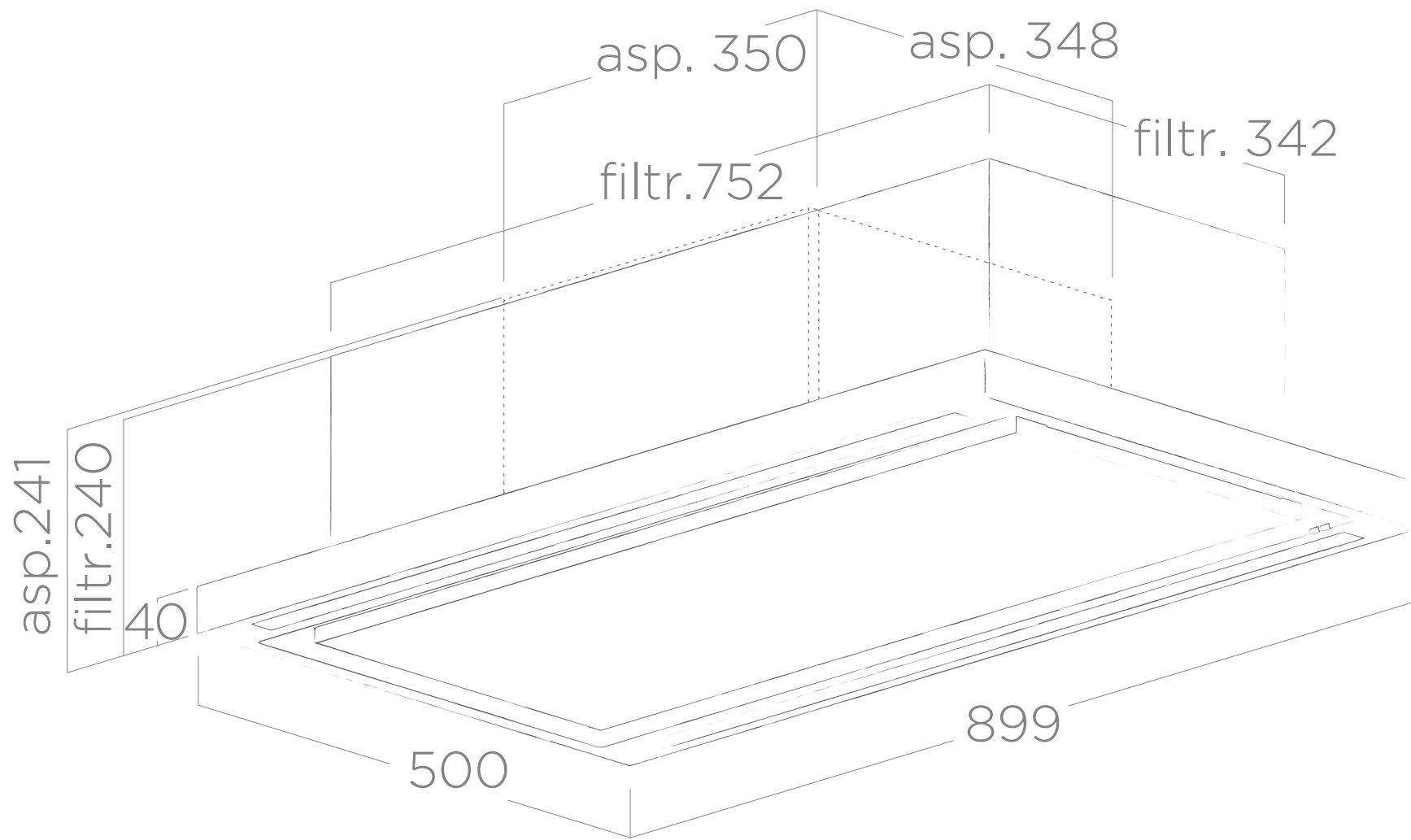
FALSE CEILING CUT: 480X880
