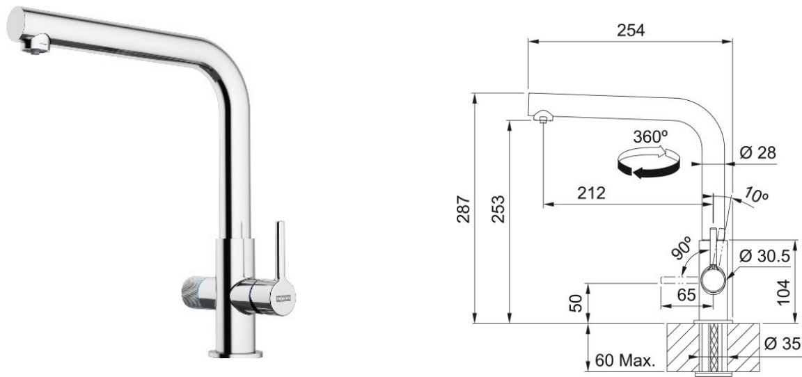
Tap Lina Clear Water 2.0 L-spout Swivel chrome, new lever
