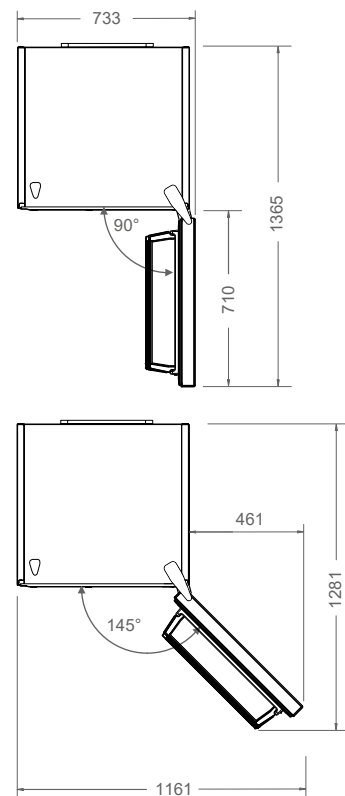
TOP VIEW
